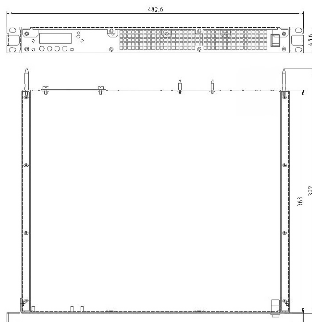
Инвертор PS48/1500(HS), PS48/1500(STS-HS)
