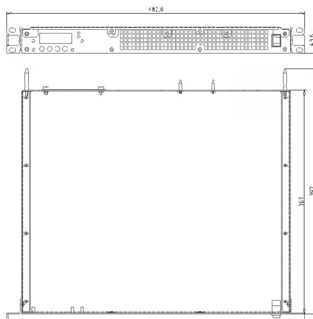
Инвертор PS48/1500(HS), PS48/1500(STS-HS)
